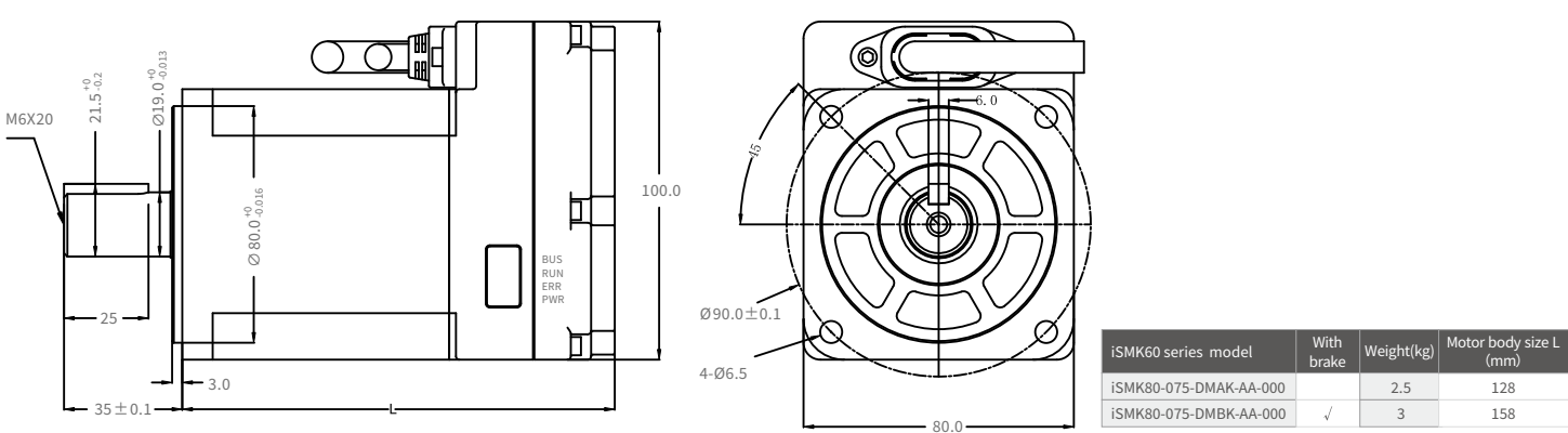
iSMK80 series mechanical dimension diagram (unit:mm)
