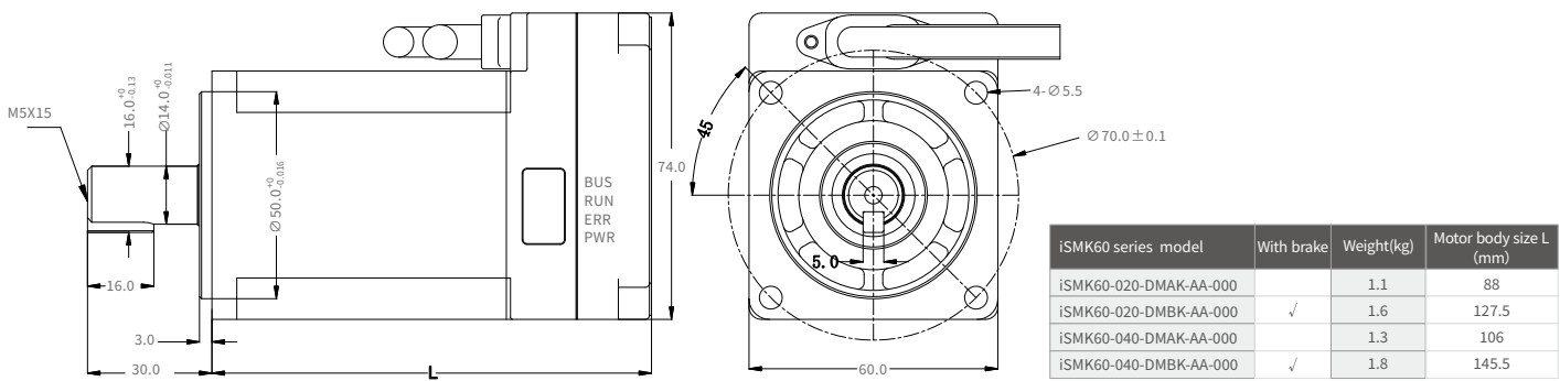
iSMK60 series mechanical dimension diagram (unit:mm)
