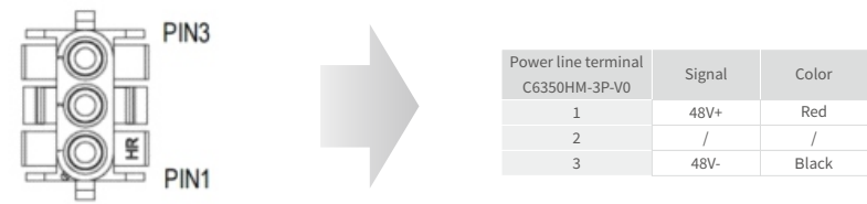
Power cable port definition
