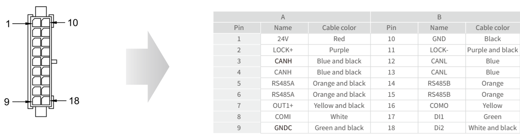
Communication cable terminal definition
