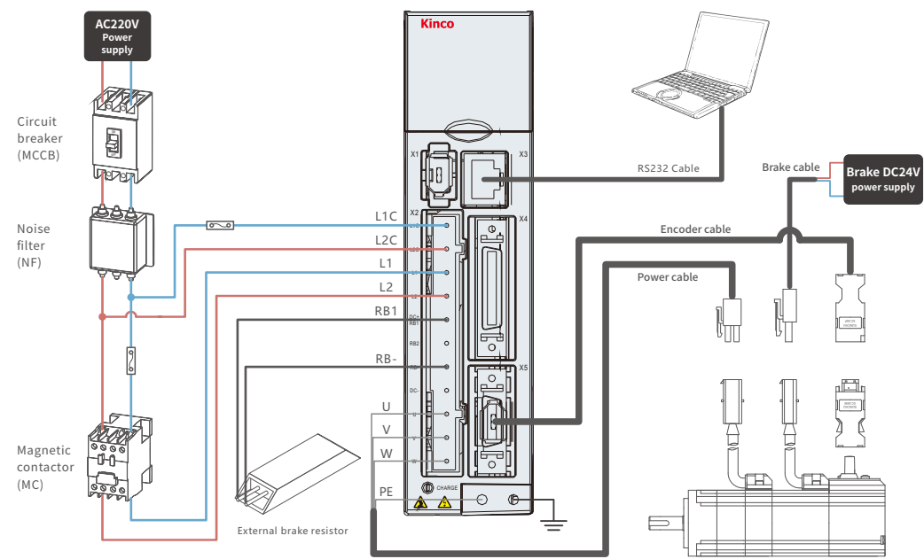
CD413/CD423/FD413/FD423 (AC220V)
