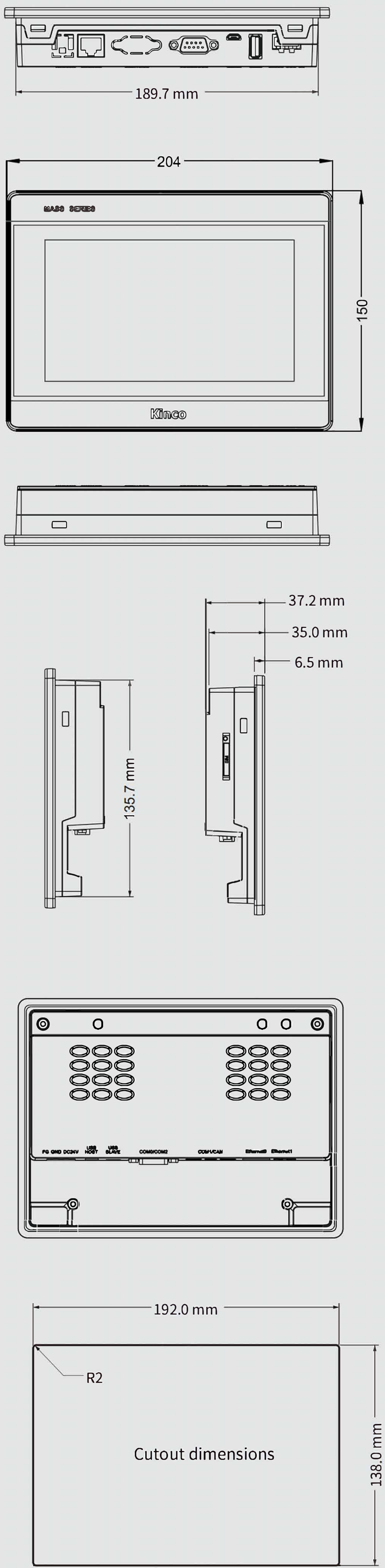
Dimensional diagram (Unit: mm)
